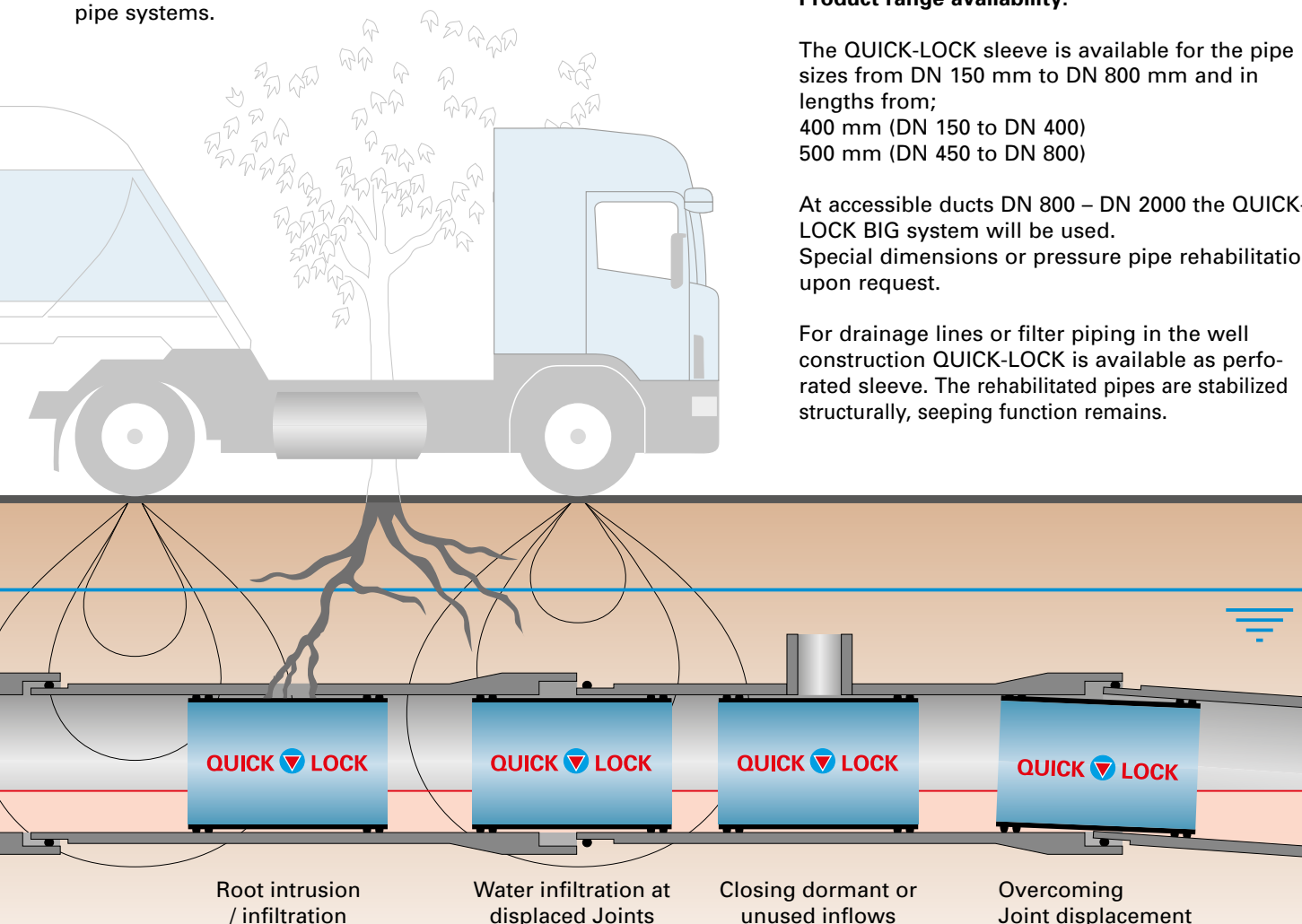
Common forms of damage found in Sewer networks
